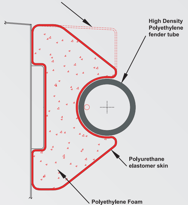
Alternative Fender Section (For Boarding Zone)
